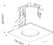
square low output
